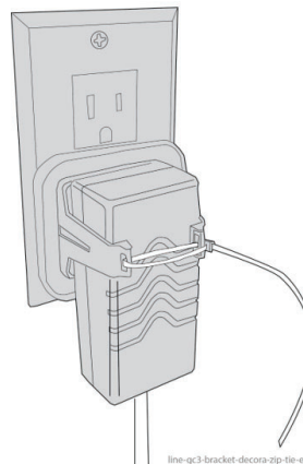
Wall Bracket Zip Tie—Decora-Style Duplex Receptacle
