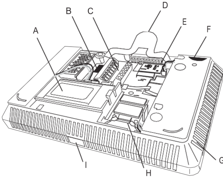
GC3 Panel - Internal Components
