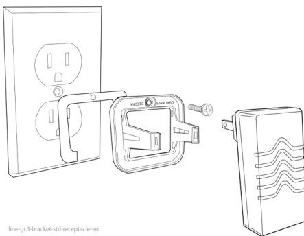
Retaining Wall Bracket—Standard-Style Duplex Receptacle
