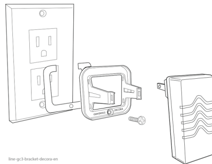
Wall Bracket Zip Tie—Decora-Style Duplex Receptacle
