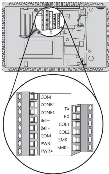
GC3 Panel—Terminal Block
