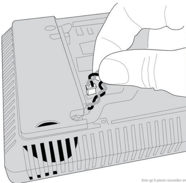
GC3 Panel—Internal Siren/Speaker Connector
