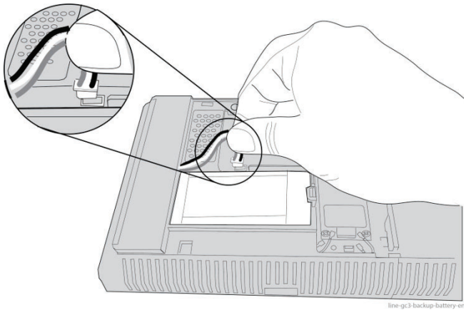
GC3 Panel—Backup Battery Connector
