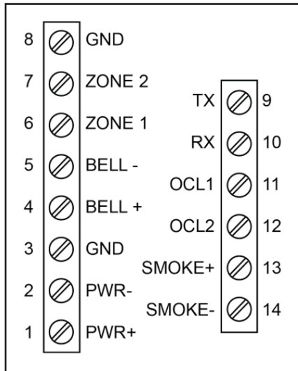
Terminal Block Positions*
