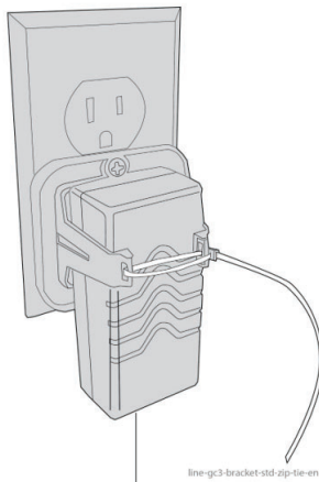
Wall Bracket Zip Tie—Standard-Style Duplex Receptacle
