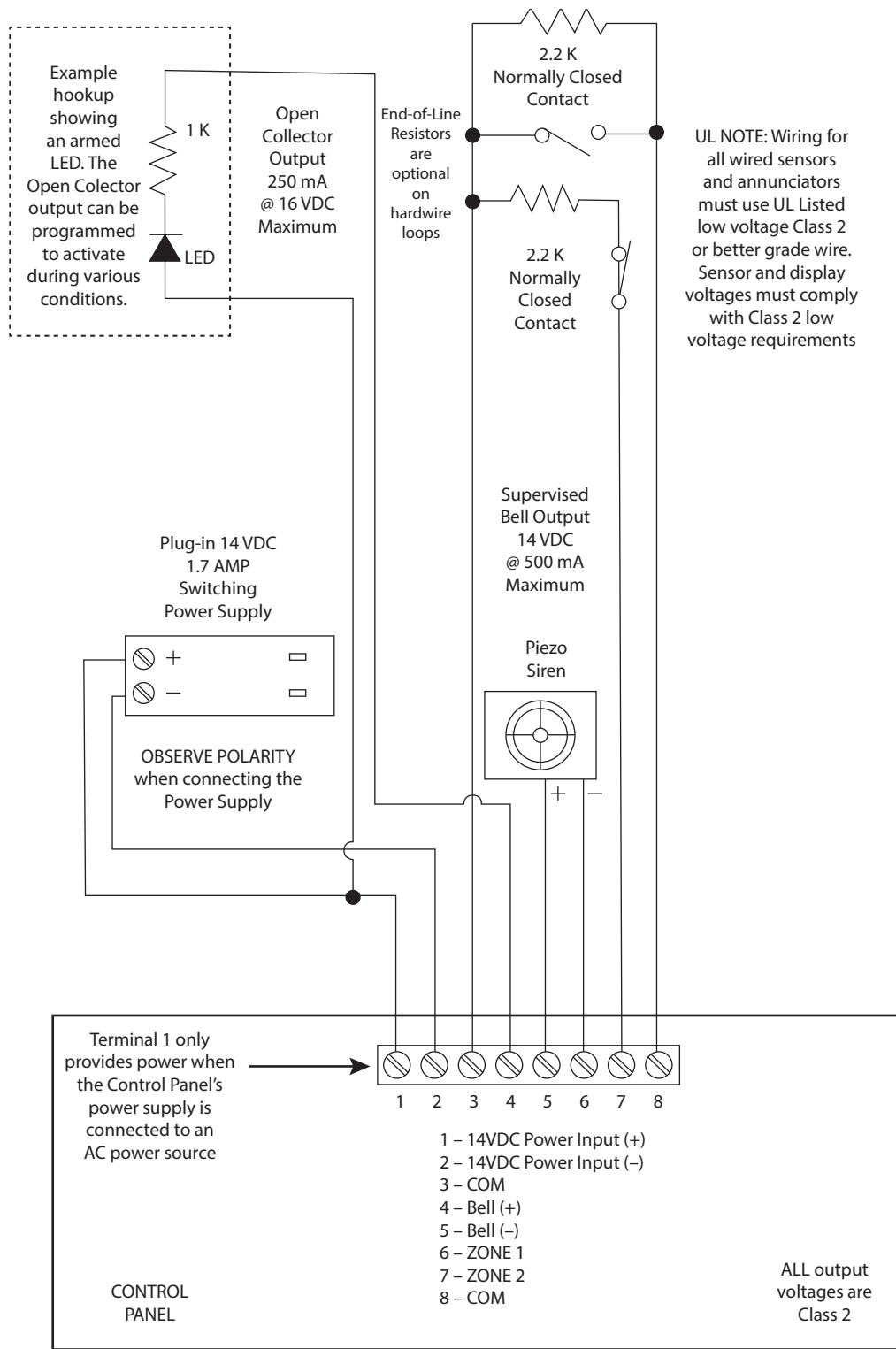
Control Panel Wiring Diagram
